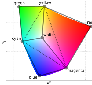
Figure 4. The projector gamut in CIELUV space, viewed from the top. The solid lines correspond to the edges of the RGB cube.
